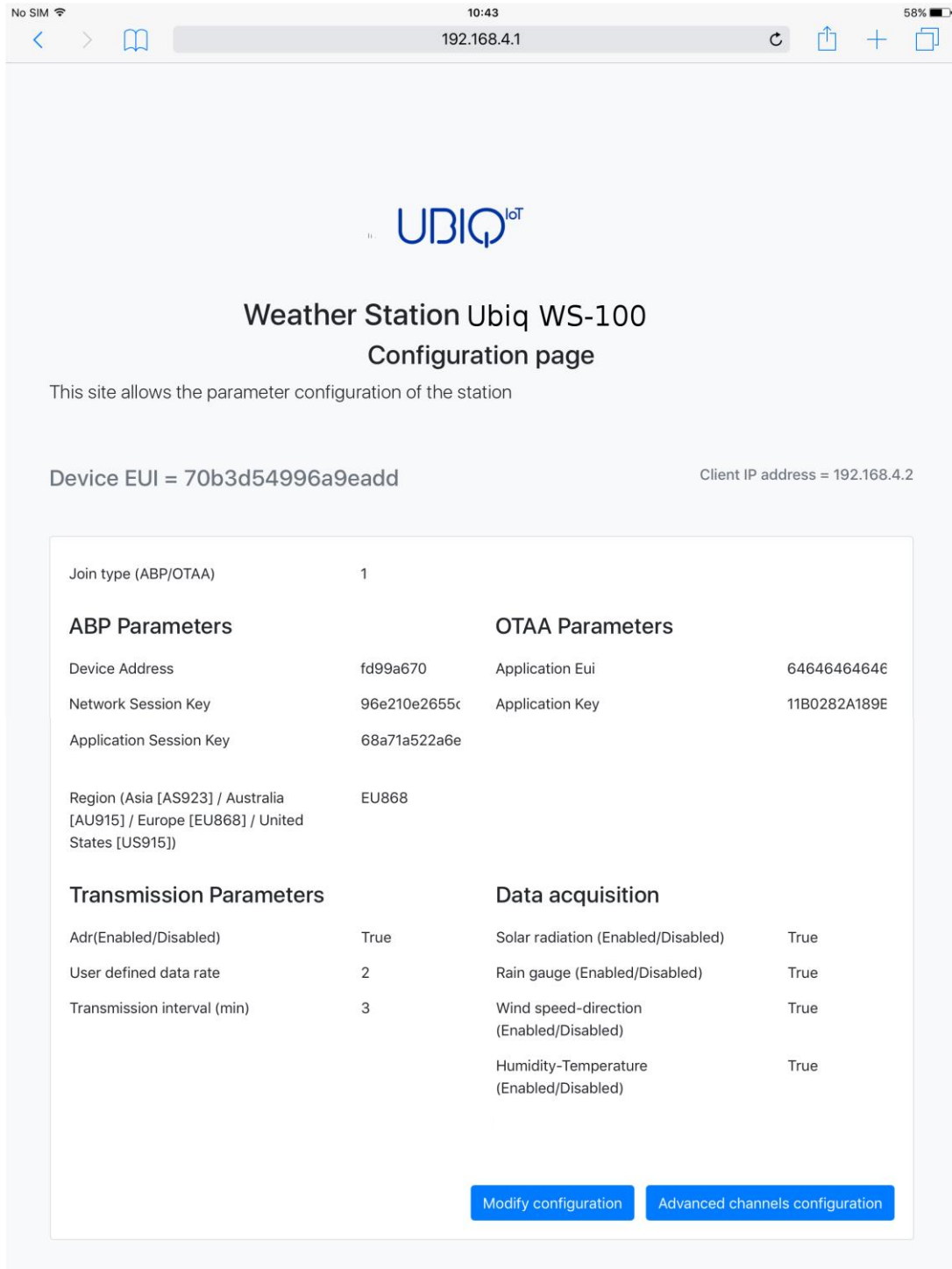
Figure 3 - Configuration page
